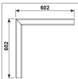
PROLINE 50 REC system coupler type L DN
