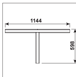
PROLINE 50 REC system coupler type T DN
